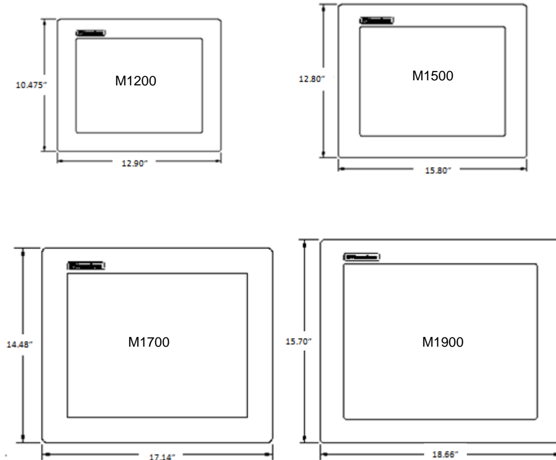
Figure 1.0: M-Series Front Panel Comparison
